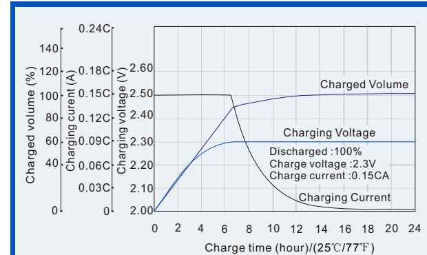
Charge characteristics (25°C, 77°F)
